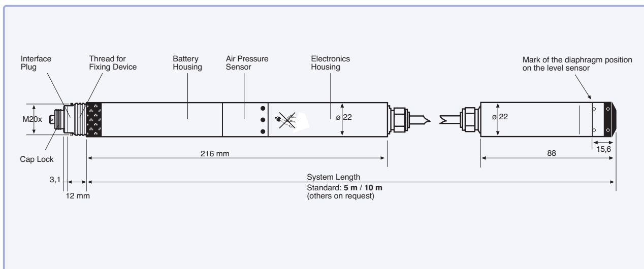
Integrated air pressure sensor with diaphragm protection
